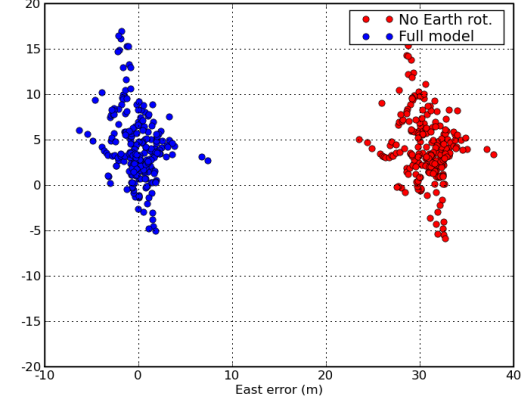
Horizontal positioning error [SPP]
