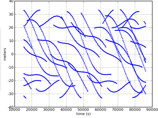
Model: Earth rotation during signal flight time [SPP]
