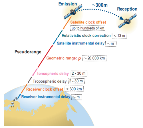
Model: Model: Sat. coord. in reception time instead of emission [SPP]
